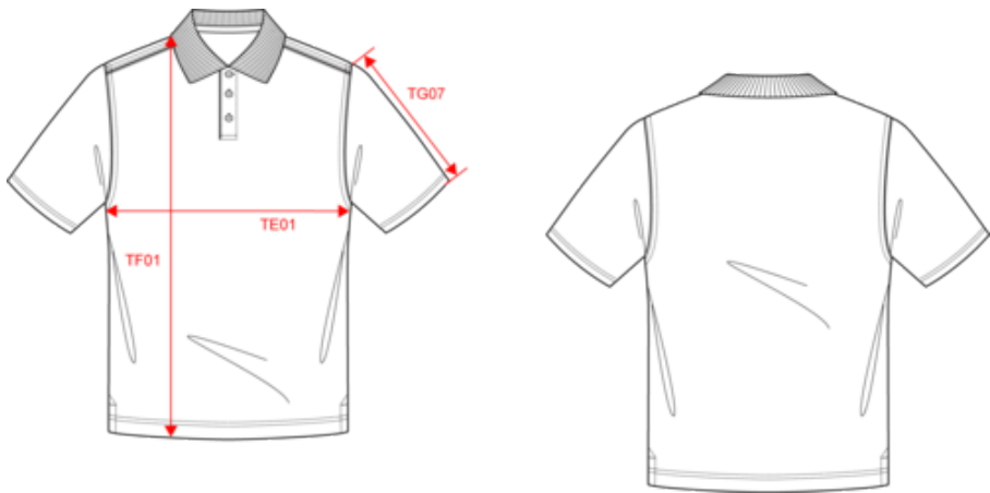
Dimensions (cm)
